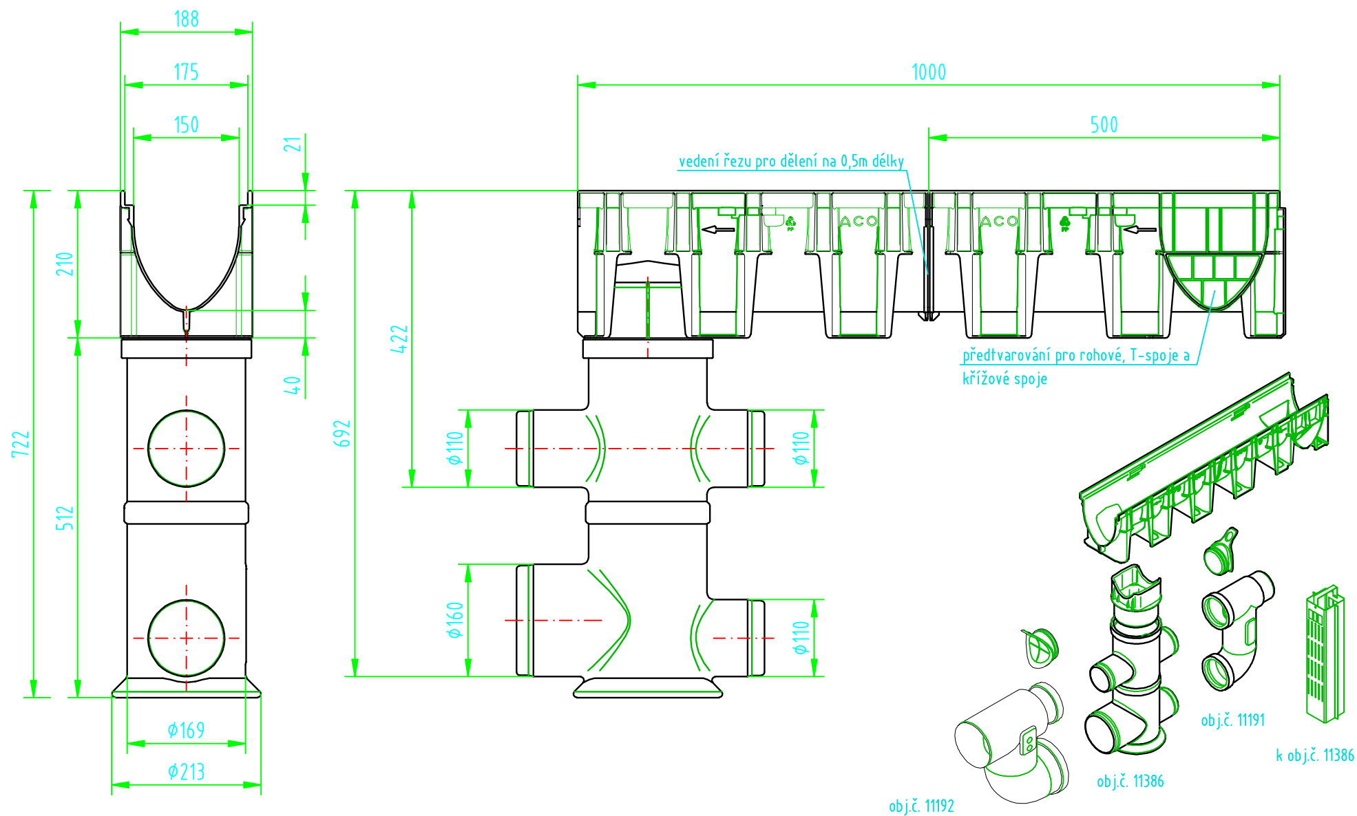
ACO DRAIN X 150 C - žlab H=210mm + vpust
